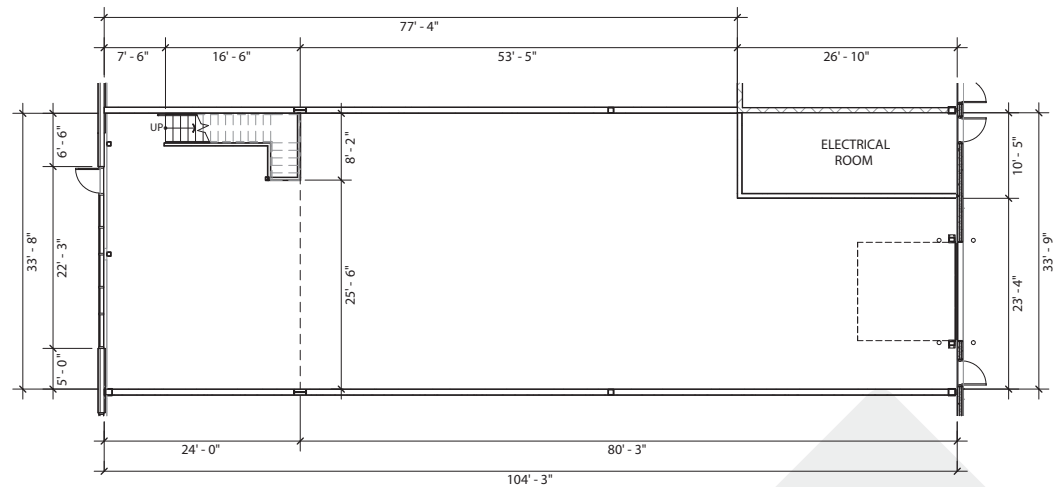
Main Floor
